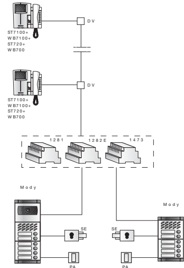
Multi-way videointercom system with 2 automatically switched entrances, one of which only audio, traditional system
