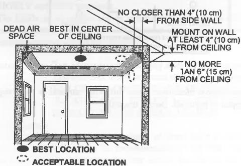
Figure 4: Recommended smoke alarm mounting locations:
